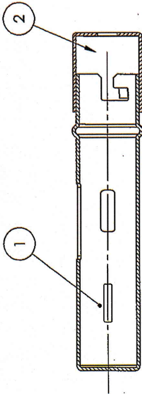
SECTION F-F
