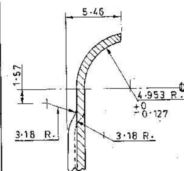
ENLARGED PART SECTION A-A.
