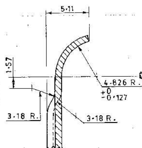
ENLARGED PART SECTION B-B.
