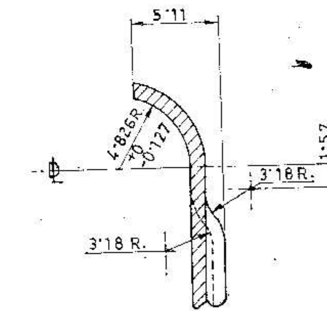
ENLARGED PART SECTION "B-B"
