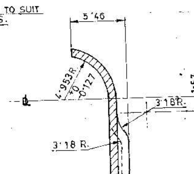
ENLARGED PART SECTION 'A-A'
