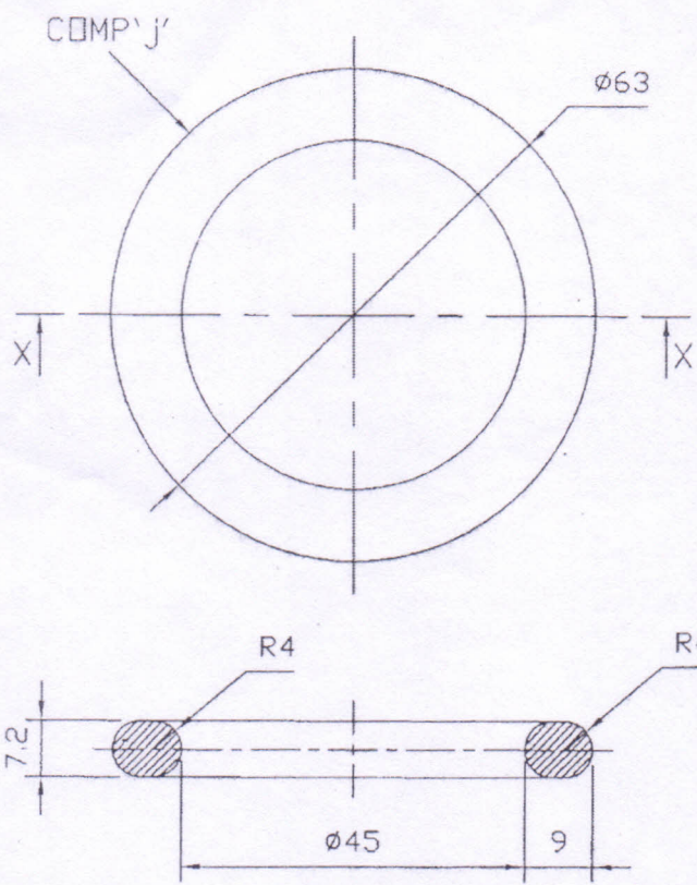
SECTION-XX 1-OFF
