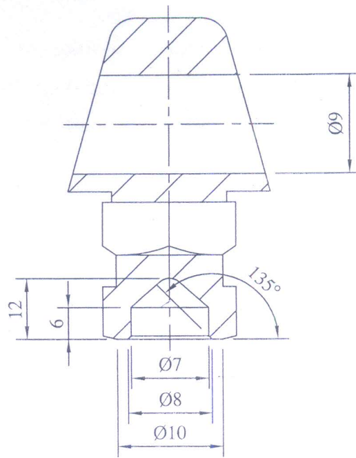
SECTION-XX SCALE 2 : 1
